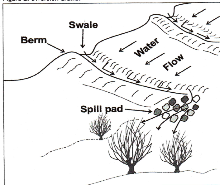
Figure 2. Diversion drains.
